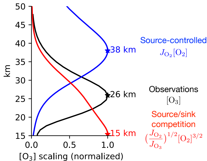
Figure 2. The vertical structure of the tropical ozone layer in observations (black) and from the scalings within the two paradigms (blue and red). Observations of O_3 are from homogenized satellite data in the SWOOSH dataset (Davis et al., 2016) averaged from 1984–2023 and over the tropics from 30^\circ\text{S} – 30^\circ\text{N} . The photolysis rates J_{O_2} and J_{O_3} are calculated based on optical depth-based radiative transfer with overhead sun and absorption by O_2 and O_3 (using the observed profile), otherwise following the methods in Section 2. All profiles are normalized by their maximum value, whose altitude is starred and labeled.
