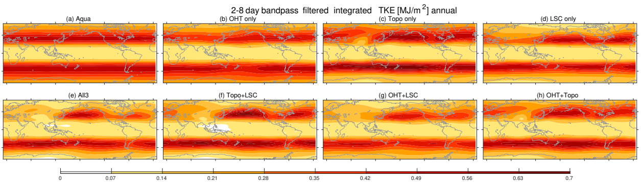
Figure 5. Two to eight day bandpass filtered transient kinetic energy (equation 1) for each of the runs described in Table 1.
