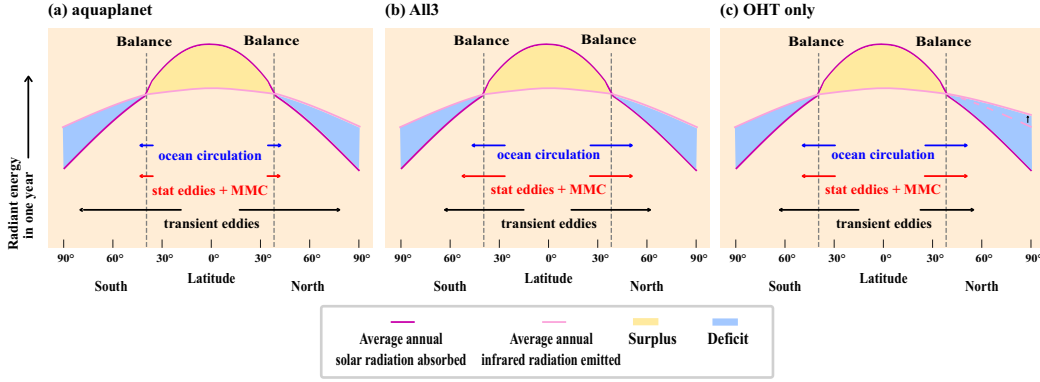
Figure 4. Schematics of the energy budget response in (a) aquaplanet; (b) ALL3; (c) in OHT only. In all configurations, the shortwave term (dark pink) is similar, however the longwave term in (c) is higher in the NH than in aquaplanet (see dashed curve in c) due to NH surface warming enlarging the energy deficit in the NH extratropics, which then requires an increase in the total NH meridional heat transport. This partially mitigates the effect of stationary eddies and ocean circulation which in isolation induce a weaker NH storm track compared to aquaplanet.
