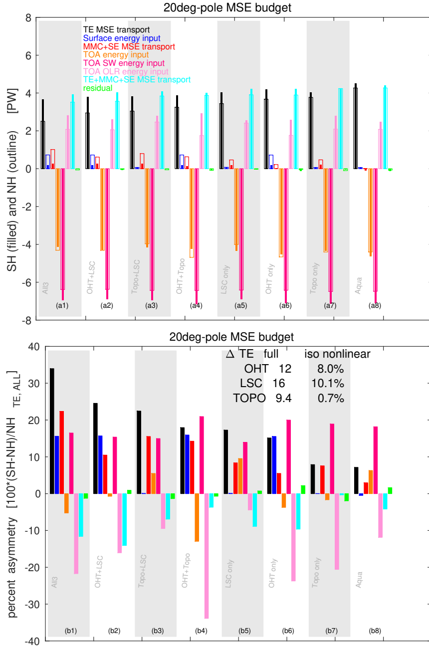
Figure 9. Moist static energy budget averaged from 20^\circ to the pole (equation 2). In panel (a), we show each term for the SH (narrow filled bar) and NH (wide outline-only bar) separately, and in panel (b) the percent difference with the transient term in the NH taken in the denominator (e.g., the OLR percent difference is \frac{OLR_{SH} - OLR_{NH}}{TE_{NH}} ). For simplicity in our plots we lump together \Delta MMC with \Delta SE . Panel b also summarizes the NH vs. SH asymmetry in sub-monthly MSE flux in response to each surface inhomogeneity for both the isolated and full nonlinear responses. A similar figure but for the White et al. (2021a) configuration is shown in Supplemental Figure S5.
