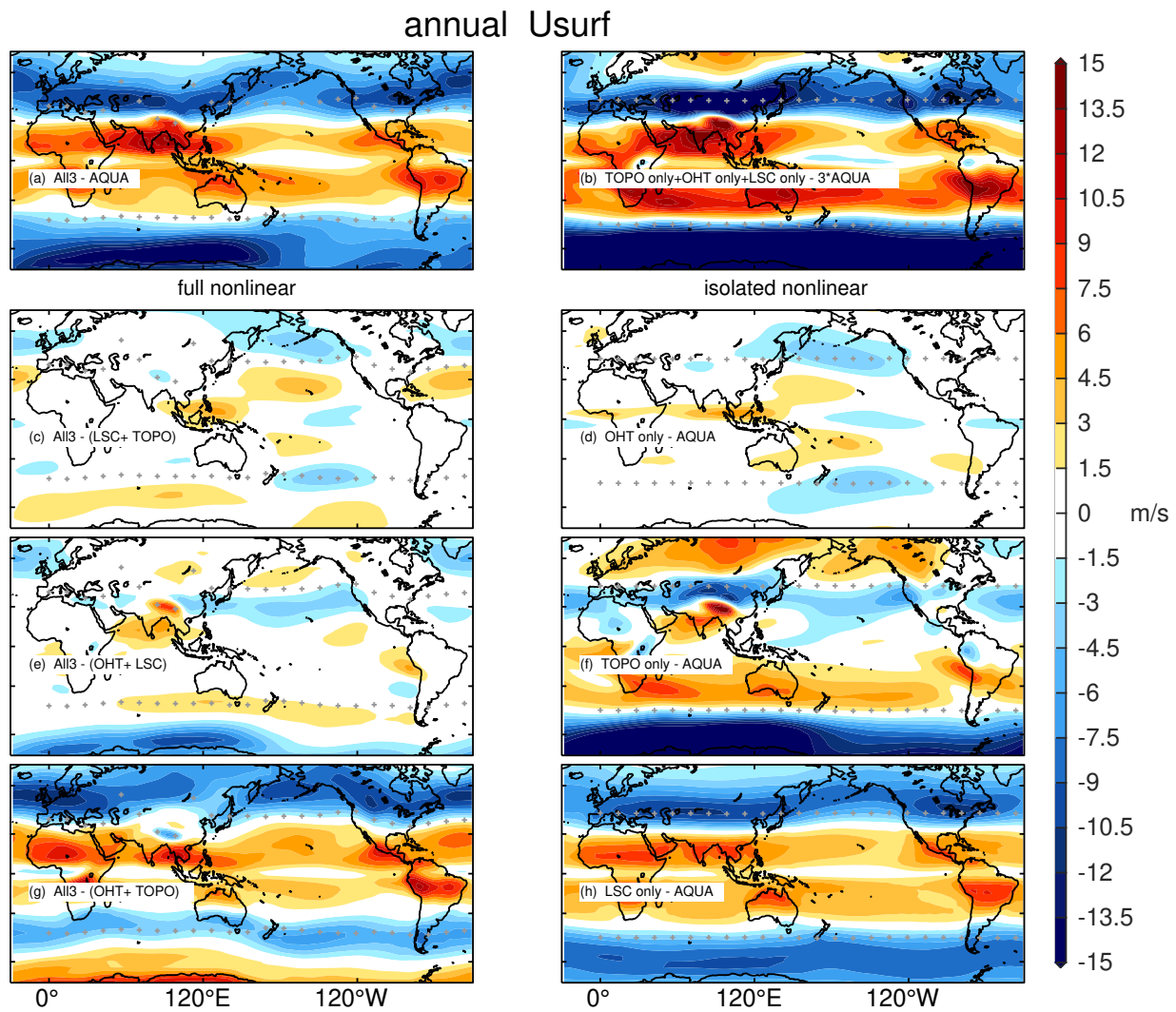
Figure 14. As in Figure 6 but for zonal wind at the lowest atmospheric model level. The contour interval is 1.5m/s. Gray stars indicate the climatological jet maximum in (left) All3 and (right) AQUA.
