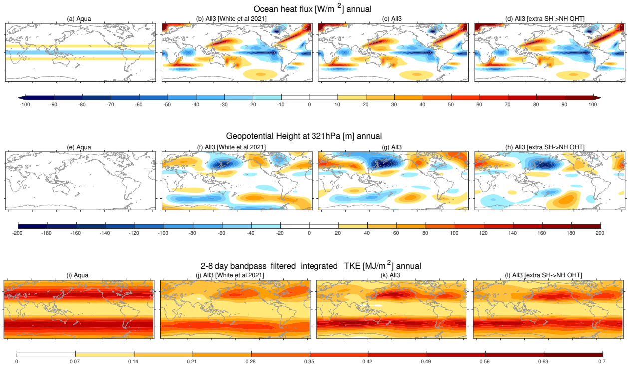
Figure 3. Ocean heat flux used for the (a) aquaplanet configuration (Merlis et al., 2013); (b) the All3 configuration of White et al. (2021a); (c) the updated All3 configuration used in this paper (see equation B1); (d) as in (c), but with an amplitude factor of 3.5\text{W/m}^2 instead of 2.1\text{W/m}^2 in equation B1. Note that differences among panels (b) to (d) are hard to detect by eye, but are present in the Southern Ocean and North Atlantic. The corresponding stationary wave structure for each configuration is shown in the second row, and the TKE in the third row.
