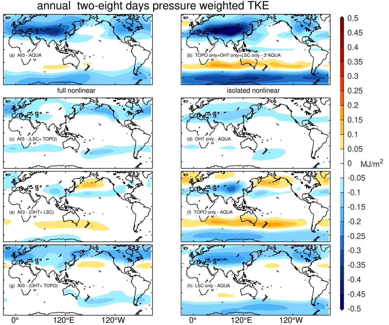
Figure 6. (a) Annual averaged and pressure integrated transient kinetic energy after bandpass filtering u and v for 2 to 8 days (Equation 1) in ALL3 minus Aquaplanet. (b) As in (a), but for the sum of integrations with topography only, land–sea contrast only, and ocean heat transport only, each compared to aquaplanet. (c) The difference between ALL3 and the integration with land–sea contrast and topography. (d) The integration with only ocean heat transport as compared to aquaplanet. (e) The difference between ALL3 and the integration with ocean heat transport and land–sea contrast. (f) The integration with only topography as compared to aquaplanet. (g) The difference between ALL3 and the integration with ocean heat transport and topography. (h) The integration with only land–sea contrast as compared to aquaplanet. Supplemental Figure S3 shows the analogous figure but for a submonthly filter.
