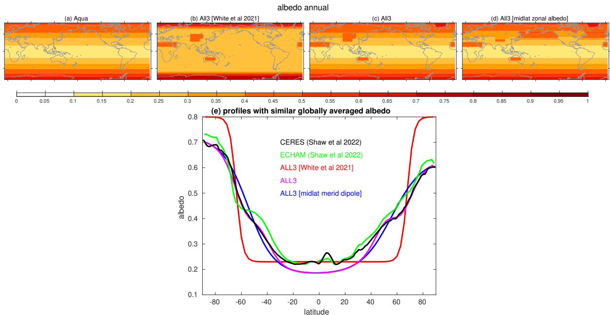
Figure 2. Albedo profiles used in this paper. CERES satellite based albedo is shown in black, and the ECHAM profile from Shaw et al. (2022) with all surface inhomogeneities is in green. The albedo profile from White et al. (2021a) is in red, and also is shown in panel (b), and the storm tracks that arise when using this profile are too weak as compared to ERA5 as discussed in Section 3. The updated albedo profile is shown in magenta, and a map view in panel (c); this albedo configuration is used in all runs with land-sea contrast. The albedo for the aquaplanet experiment is shown in panel (a), and this profile is also used in runs without land-sea contrast. Section 6 discusses two sensitivity ALL3 runs where we alter the albedo: the albedo for the case in which we add land-ocean albedo differences is shown in panel (d), and the albedo for the case in which the meridional dipole of equation A2 is not included is shown in blue in panel (e). Note that the albedo in MiMA refers to surface albedo, while in CERES and ECHAM it refers to top of atmosphere albedo.
