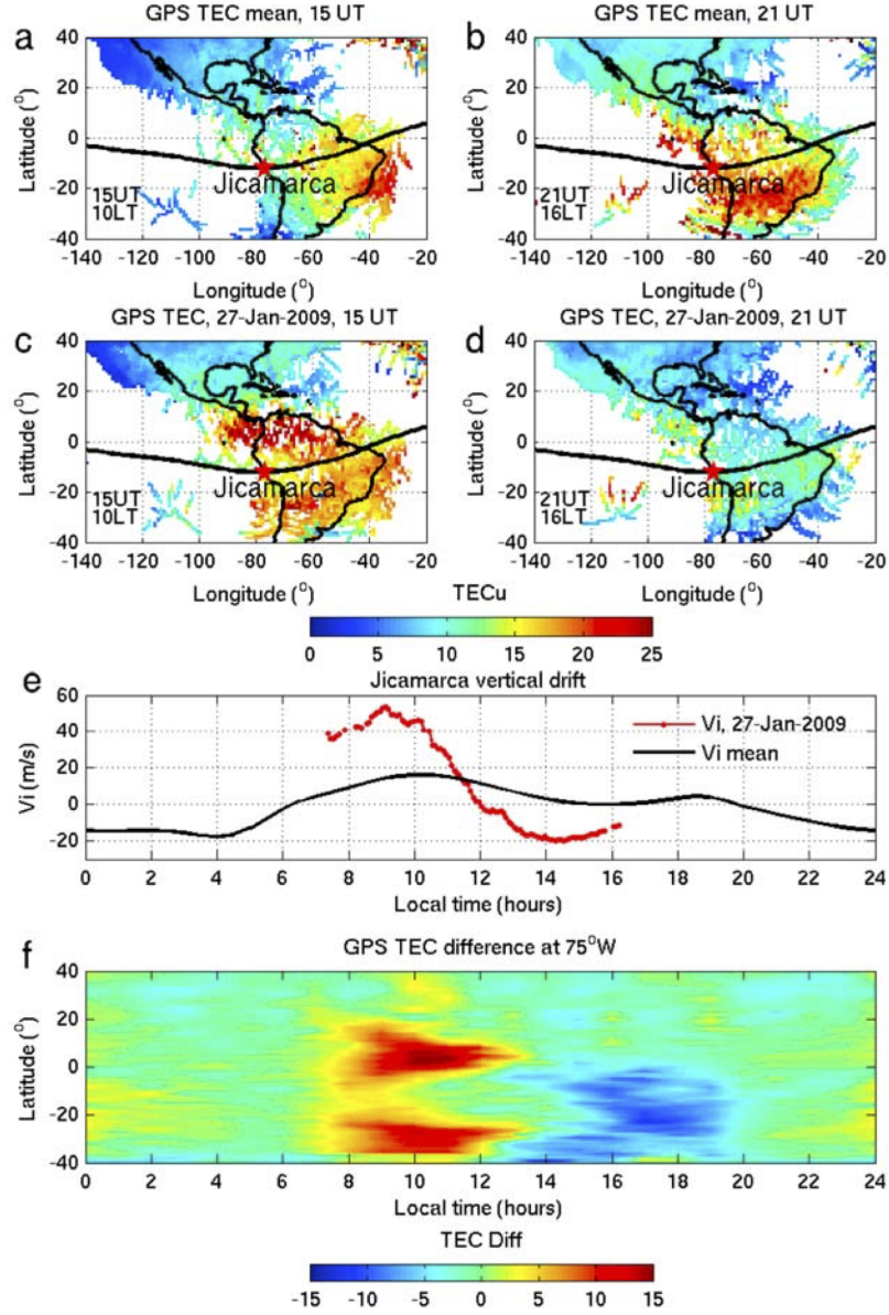
Figure 10. Observations of ionospheric behavior during the 2009 SSW event. (a) Mean total electron content (TEC) at 15 UT (morning sector, 10LT at 75°W). (b) Same as Figure 10a, except for at 21 UT (afternoon sector, 16 LT at 75°W). (c) TEC in the morning sector (15 UT) on January 27, 2009, during the SSW. (d) TEC in the afternoon sector (21 UT) on January 27, 2009. (e) Vertical drift observations by the Jicamarca incoherent scatter radar (12°S, 75°W) at 200-500 km altitude. The red line indicates observations on January 27, 2009, and the black line indicates the average behavior for winter and low solar activity. (f) Change in TEC at 75°W during the SSW as a function of local time and latitude. From Goncharenko, Chau, et al. (2010).
