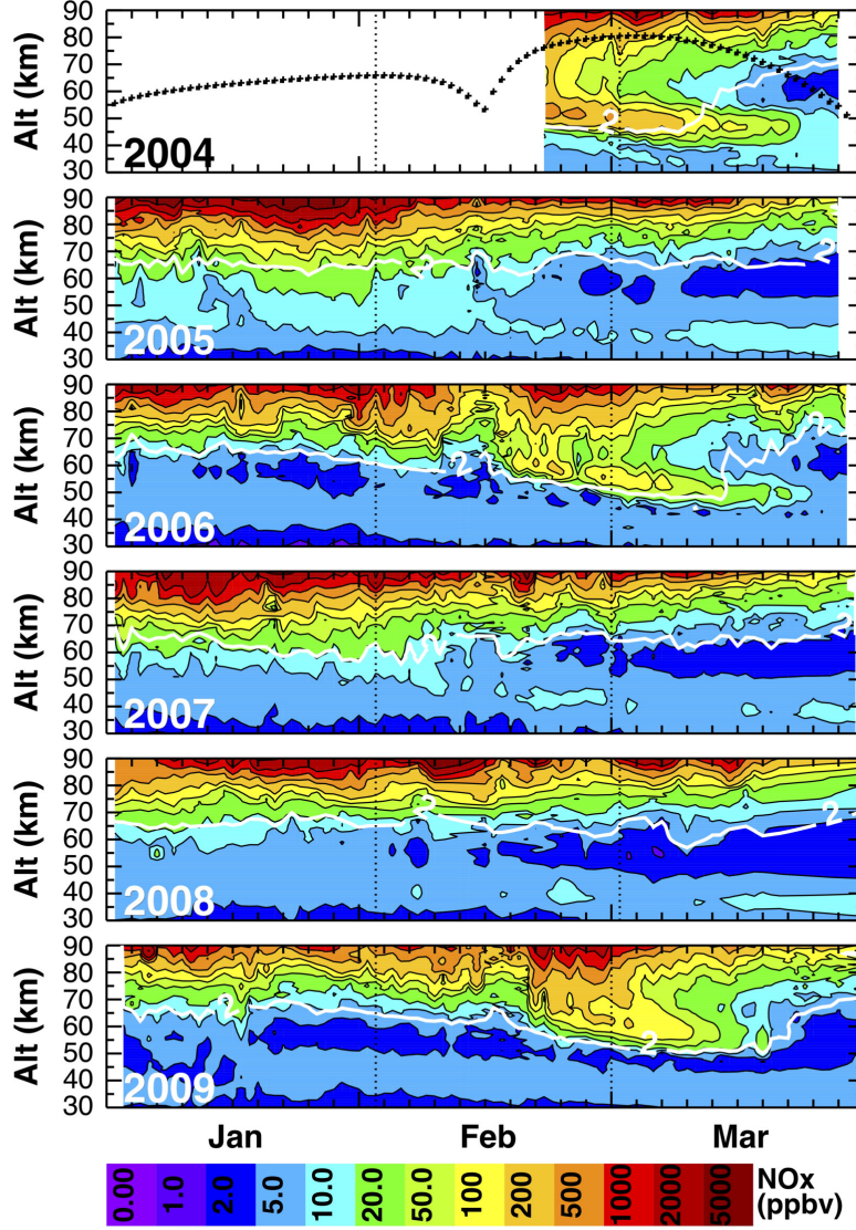
Figure 9. Zonal average ACE-FTS NO x (color) in the NH from 1 January through 31 March of 2004-2009. The white contour indicates CO=2.0 ppmv. Measurement latitudes are shown in the top panel as black dots. From Randall et al. (2009).
