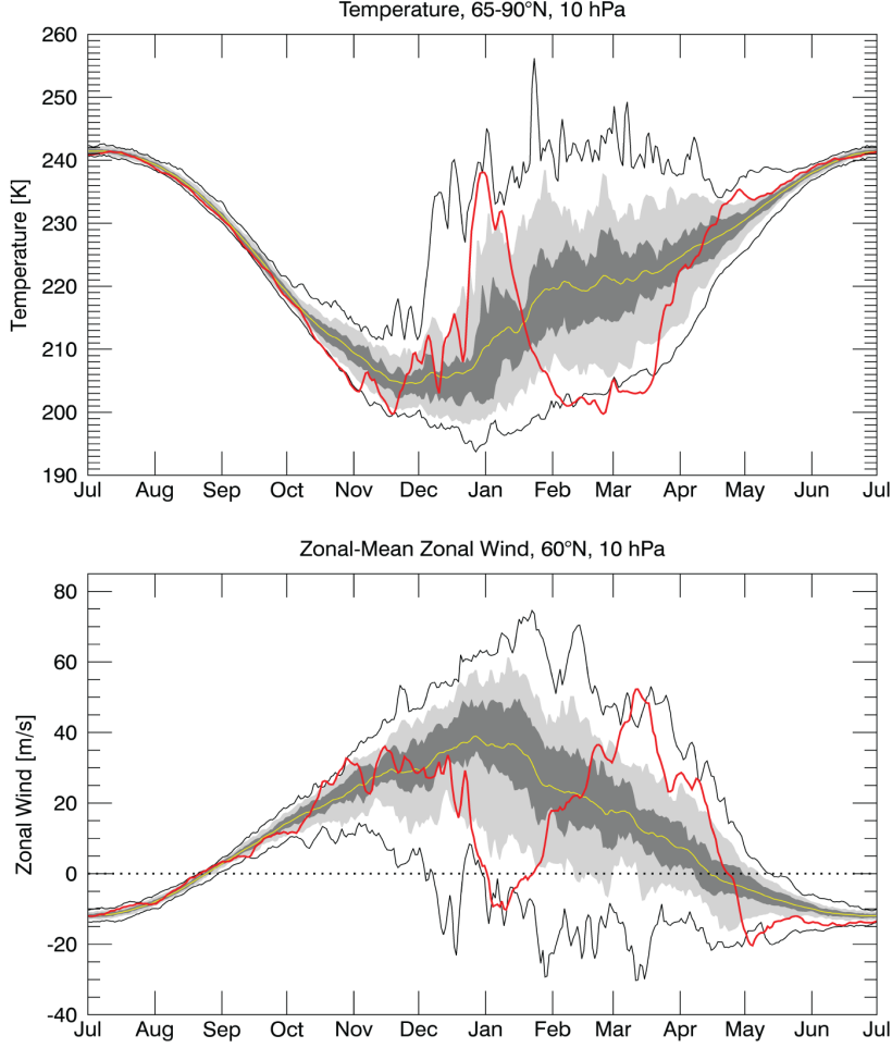
Figure 1. 10-hPa 65°–90°N ERA-Interim reanalysis (Dee et al., 2011) zonal-mean temperatures (top) and zonal-mean wind at 60°N (bottom) for July 2018–June 2019 (red lines). An SSW event is seen as the upward spike in temperature and the reduction to less than 0 m/s in zonal wind (easterlies). The yellow lines signifies the average conditions in the stratosphere for that time of year, while the gray shading show 70th (dark) and 90th (light) percentiles. Solid black lines show the max/min for prior winters 1979–2018. The month ticks indicate the first day of the month.
