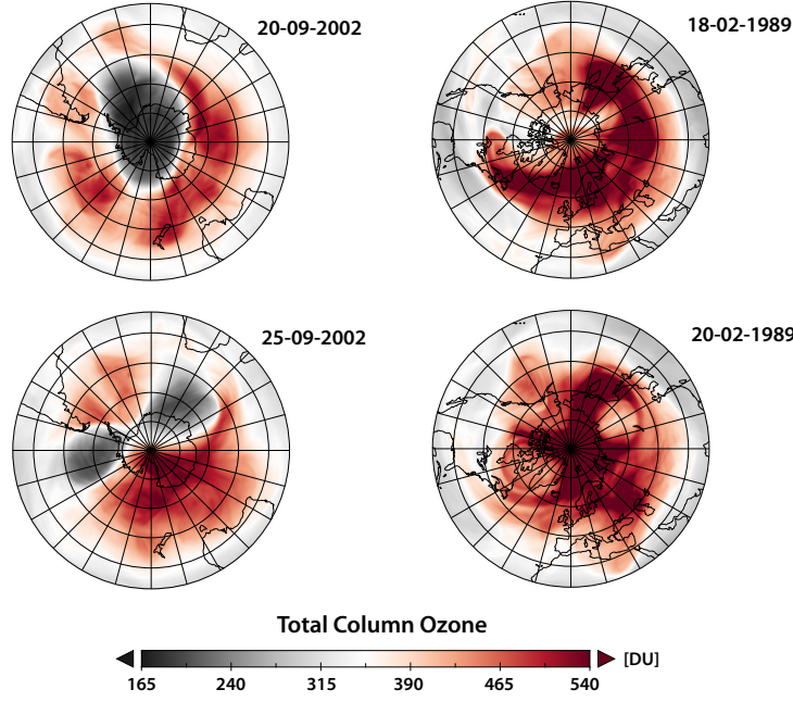
Figure 11. Total column ozone distributions in [DU] as obtained from ECMWF ERA5 before (upper panels) and after (lower panels) SSW events, for the Antarctic polar region in 2002 (left column) and the Arctic polar region in 1989 (right column), respectively.
